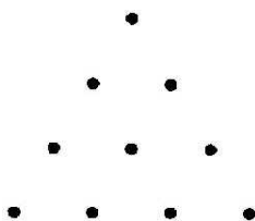
Figure 2. The tetractys.
