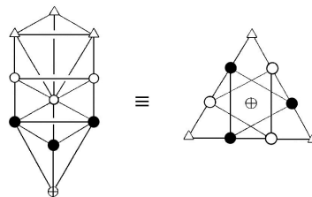
Figure 3. Equivalence of the Tree of Life and the tetractys.
