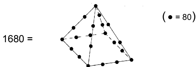
Figure 15. The edges of the square pyramid embody the superstring structural parameter 1680.
