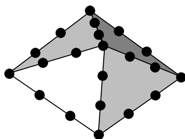
Figure 13. 21 yods lie on the edges of a square pyramid.
