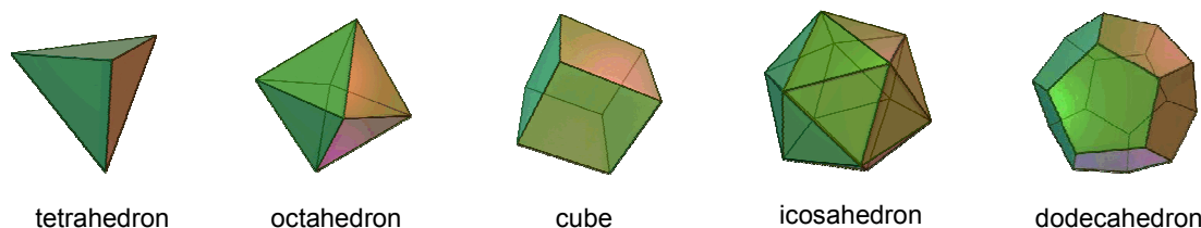
Figure 9. The five Platonic solids.
