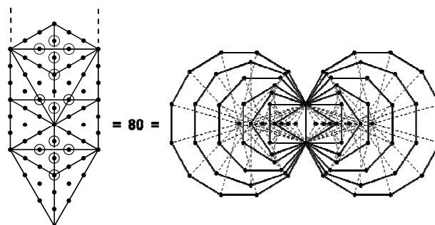
Figure 8. The 1-tree has as many yods (80) as the 94 sectors of the (7+7) enfolded polygons have corners.
