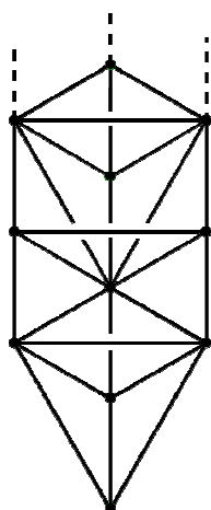
Figure 4. The 1-tree.
