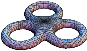
Figure 26. The 3-torus.
