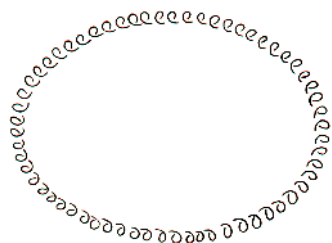
Figure 2. The 1680 turns of a helical whorl.
