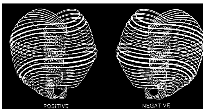
Figure 1. The two chiral forms of the building block of matter, according to the micro-psi vision of Besant & Leadbeater (from Occult Chemistry , 3rd ed., 1952).
