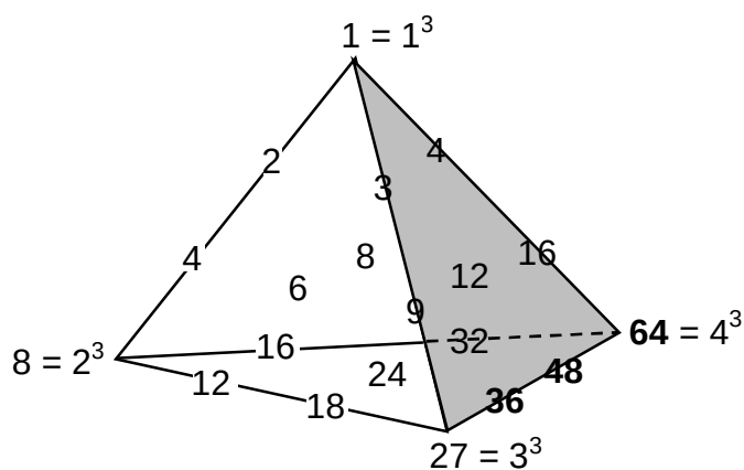
Figure 30. The 70 polygons enfolded in the 10-tree have 350 corners not shared with polygons enfolded in the 11th Tree of Life. This is the sum of the 20 integers in the tetrahedral Lambda Tetractys. Assigning the Decad to these 350 corners generates the number of hexagonal yods in each half of the two concentric polyhedra in the polyhedral Tree of Life.
