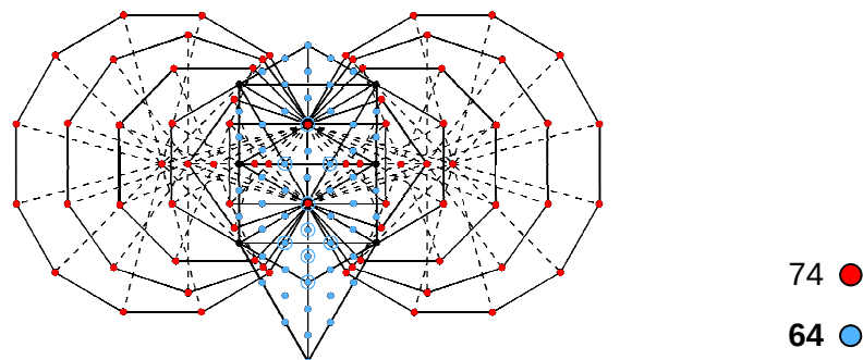
Figure 18. The inner & outer Trees of Life have 138 yods/corners that are unshared with each other. They denote the 138 vertices of the 660 triangles in their polyhedral counterparts.
