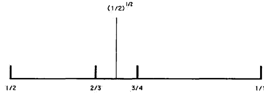
Figure 3: The octave interval, defined by the notes of frequency 1/2 , the tonic, and 1/1 , its superior octave, is divided by its geometric mean \sqrt{1/2} as shown. The interval is defined by the first two convergents of the golden number, 1/1 and 1/2 , to which we have added the next convergent, 2/3 . However, this breaks the symmetry of the scale. There exists another solution which consists of the permutation of the short and long intervals defined by 2/3 , i.e. 3/4 . This solution can be viewed as that symmetric to 2/3 through the symmetry axis \sqrt{1/2} . Symmetry is meant here in the Greek sense, that is, as an equality of ratios, i.e. (2/3)/\sqrt{1/2} = \sqrt{1/2}/(3/4) . If we take logarithms of all quantities the symmetry becomes the usual sort and the geometric mean, \sqrt{1/2} , can be viewed as a mirror.
