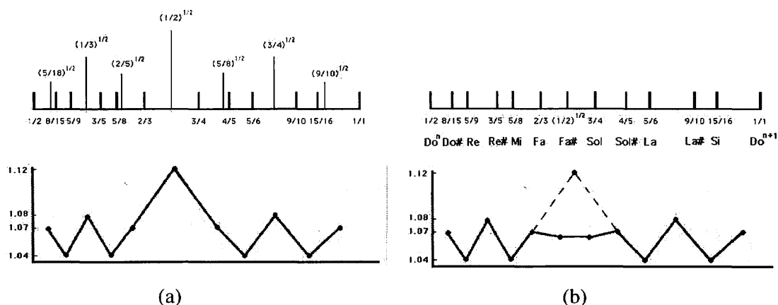
Figure 4: (a) The golden scale construction developed until the fifth convergent c_5 = 5/8 (upper panel), and the intervals between adjacent notes (lower panel). We can see that the intervals are distributed in a band. If we take as a rule that the intervals cannot be greater than the quotient of convergents c_{n-2}/c_{n+1} , in this case c_3/c_6 = (2/3)/(8/13) = 13/12 = 1.08 , or less than that of the convergents c_n/c_{n-1} , here c_5/c_4 = (5/8)/(3/5) = 25/24 = 1.04 , we find that the anomalous interval 1.13, between 2/3 and 3/4 , must be subdivided once. However there is no solution to this problem in rational numbers, because the inclusion of a rational number and its image generates at least one interval less than 1.04. The only possibility is thus to include the irrational axis \sqrt{1/2} itself. (b) The result of including the irrational axis. We can see that all the intervals are now within the previously defined band. As the number of notes coincides with the number of notes of the usual equal-tempered scale of twelve notes, we have given the same names to the notes of this golden scale.
