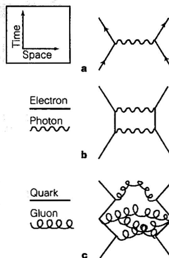
Figure 3 Feynman graphs. a, The simplest graph contributing to electron–electron scattering in QED, by exchange of a virtual photon. In a more accurate calculation, b, one must allow for multiple exchanges. c, A typical contribution to the interaction of quarks in QCD.
