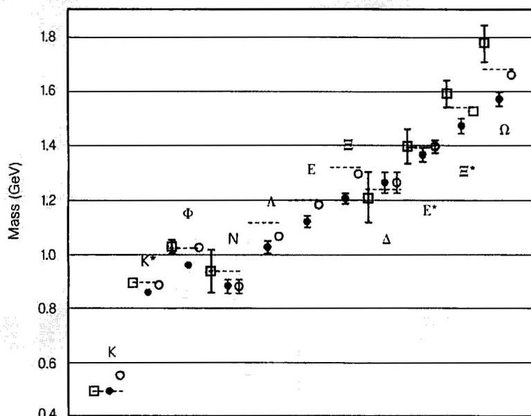
Figure 2 Comparison of masses of light hadrons (dotted lines) to various lattice simulations (data points). These calculations contain just one free parameter, the strange quark mass. Sources of error in the current lattice calculations, which are believed to be responsible for the small residual errors, are discussed in ref. 3.
