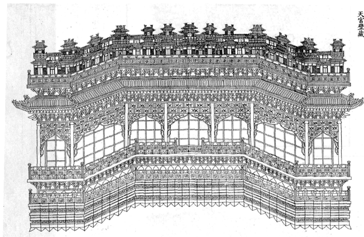
Fig. 3: Representation of a wall library; Li Jie (c. 1065–1110?), Yingzao fashi ('Construction Methods'), ed. Wanyou wenku 1933.
