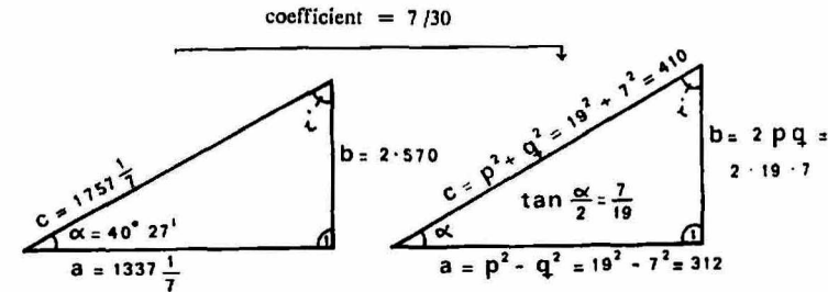
Fig. 6. The two triangles for the fourth motion of Venus
