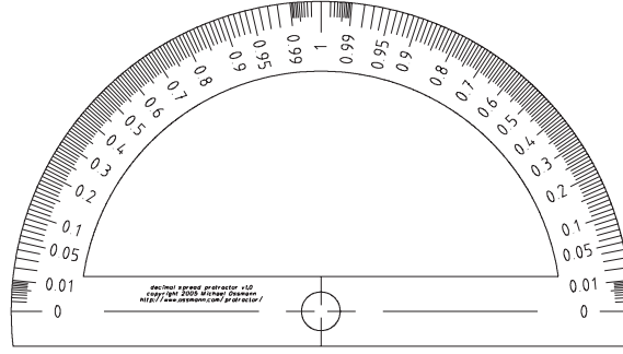
A spread protractor
