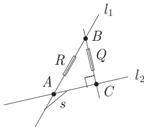
Spread s between two lines l_1 and l_2
