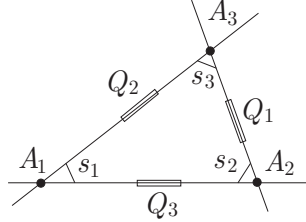
Quadrances and spreads of a triangle
