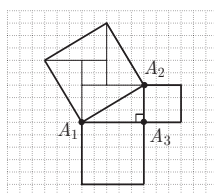
A triangle with side areas 9, 25 and 34.
