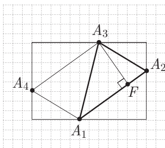
A triangle and an associated parallelogram
