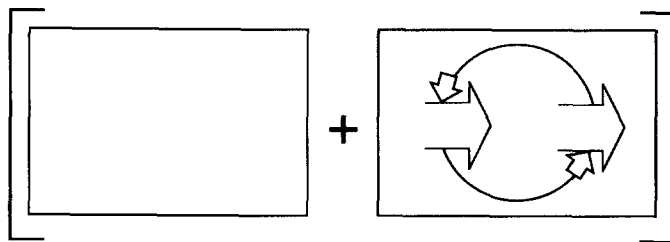
FIGURE 1 A schematic of the conjunction capturing the generalized minimal ontology of an autocatakinetic system. The left side represents the conservation out of which the autocatakinetic system and environment relation arises, and through which it is maintained. The right side shows the environment–autocatakinetic system relation. The large arrows capture the irreversible minimization of potential (the irreversible production of entropy) in the flow of the conservation (energy) from source to sink, and the small arrows capture the continuous circular relations by which the autocatakinetic system is constituted.
