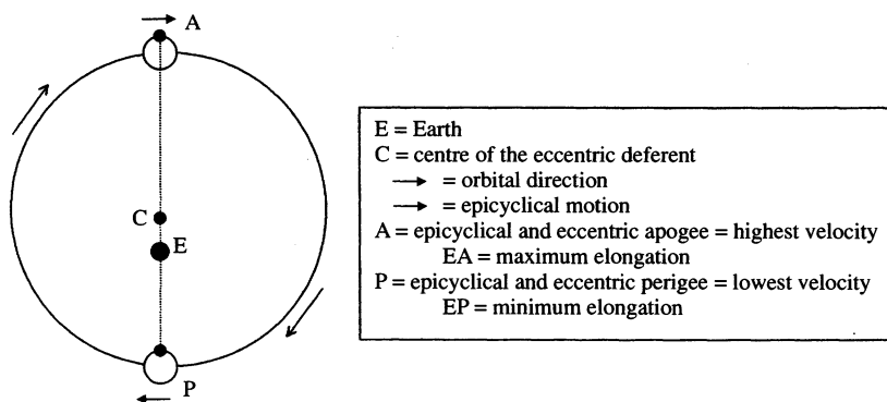
Figure 1 Planetary velocity and elongation
