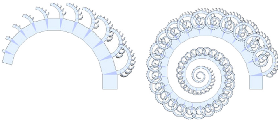
Fig. 7. Standard and greedy forms of P_{15} at i = 12 (8191 segments).
