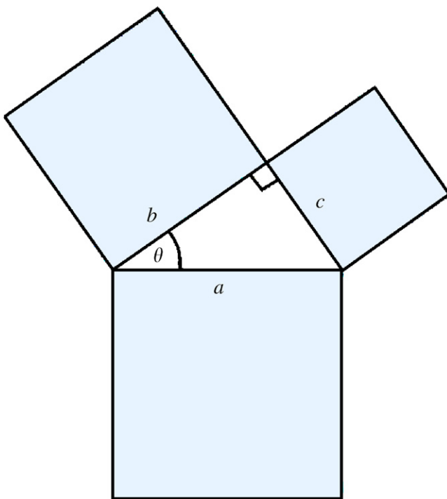
Fig. 1. Construction based upon the Pythagorean theorem.
