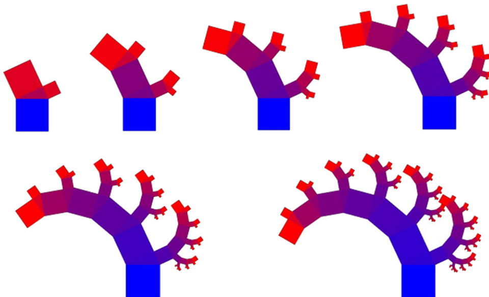
Fig. 4. Standard tree P_{25} for i = \{2, 3, 4, 5, 6, 7\} .
