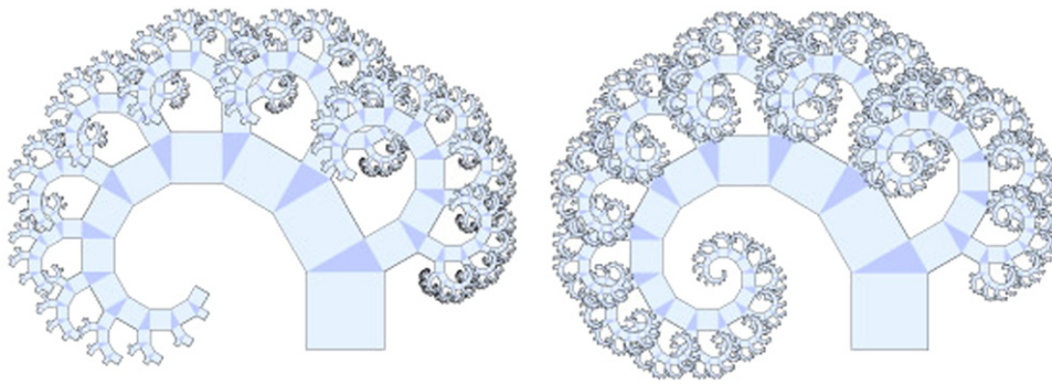
Fig. 6. Standard and greedy forms of P_{30} at i = 12 (8191 segments).
