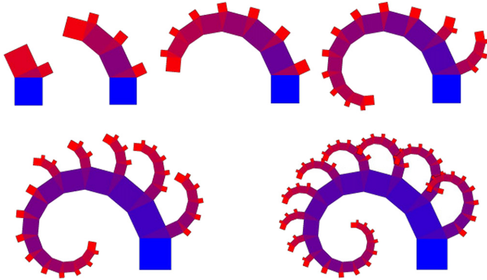
Fig. 5. Greedy tree P_{25} for i = \{2, 3, 4, 5, 6, 7\} .
