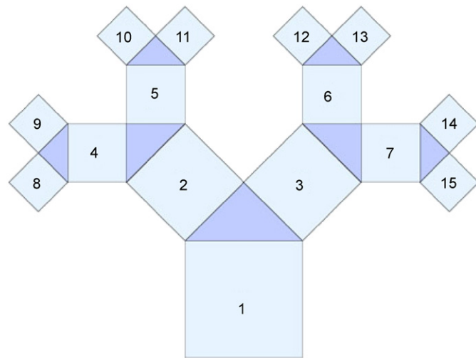
Fig. 3. Breadth-first growth order of the standard tree.
