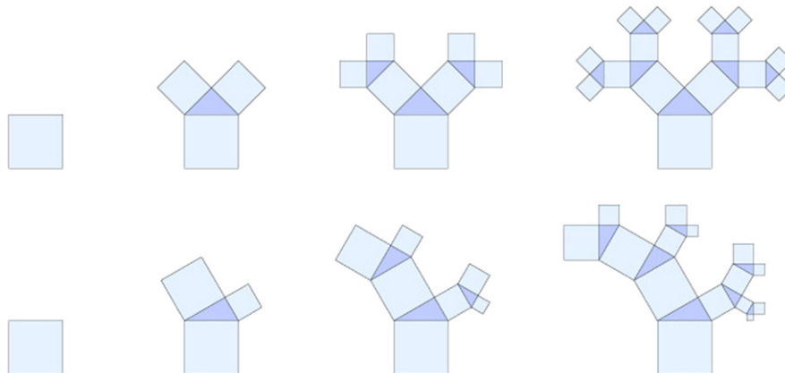
Fig. 2. First four iterations of the Pythagorean trees P_{45} (top row) and P_{30} (bottom row).
