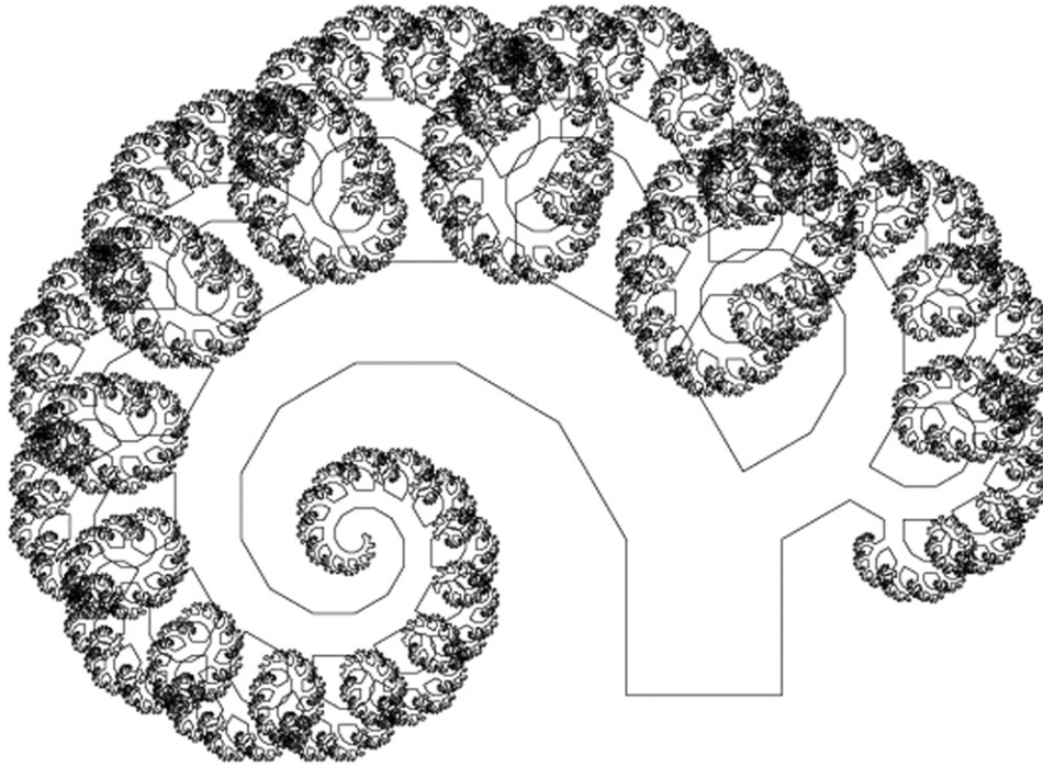
Fig. 8. Self-overlapping outline of P_{30} at i = 15 (65,535 segments) for w = 0.3 .
