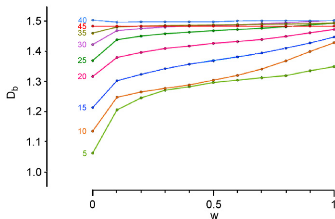
Fig. 9. Fractal dimension ( D_b ) plotted against weighting factor w for trees P_5 through P_{45} .
