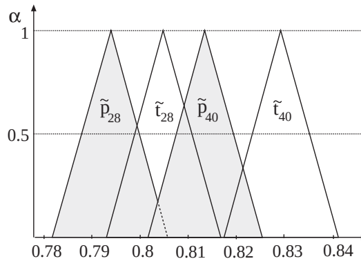
Fig. 5. Membership functions of the notes 2^{\tilde{f}_{28}}, 2^{\tilde{f}_{40}} \in \tilde{T}^{41}(\frac{1}{2 \cdot 41}) and 2^{\tilde{s}_{28}}, 2^{\tilde{s}_{40}} \in \tilde{S}_2^{41}(\frac{1}{2 \cdot 41}) .
