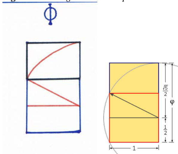
Figure 2. Starting the Golden Spiral within a Rectangle Using Euclid's Formula
