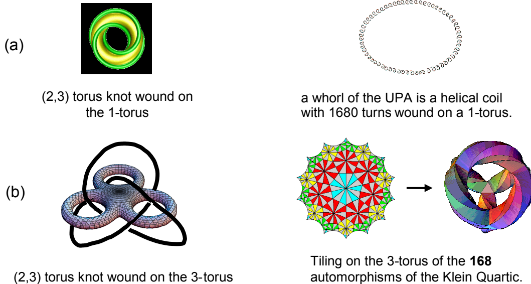
Figure 41. The 1-torus (a) on which the (2,3) torus knot winds is the surface around which each whorl of the heterotic superstring coils 1680 times. The knot can also wind around a 3-torus (b), which is the surface in which can be embedded the Klein Configuration representing the Riemann surface of the Klein Quartic with 168 automorphisms denoted by the triangular sectors of 24 heptagons.
