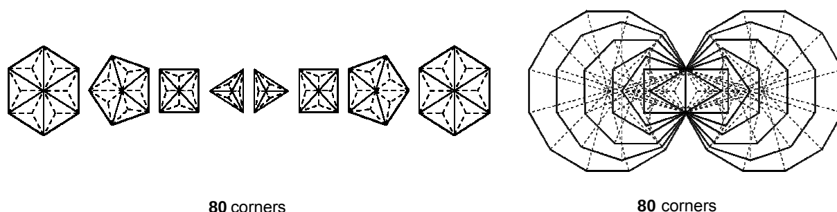
Figure 18. The 102 triangles in the (4+4) separate Type B polygons have 80 corners. They are the counterpart of the 80 corners of the 94 sectors of the (7+7) enfolded Type A polygons of the inner Tree of Life.
