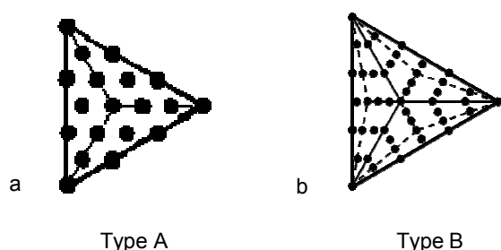
Figure 1. Type A & Type B triangles.
