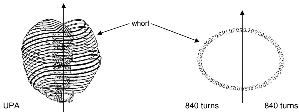
Figure 14. The UPA, the unit of matter described by Besant & Leadbeater, is the E_8 \times E_8 heterotic superstring. It consists of 10 closed curves, or "whorls," each a helix with 1680 circular turns. Every whorl winds 2\frac{1}{2} times around the spin axis of the UPA in an outer helical spiral of 840 turns and returns to its top by twisting 2\frac{1}{2} more times in a tighter, inner spiral of 840 turns.
