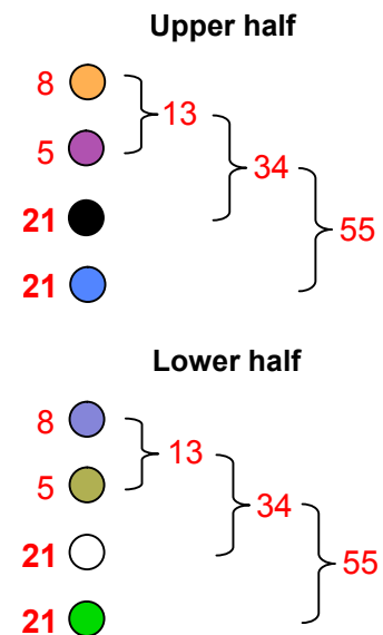
Figure 8. The Fibonacci number pattern in each half of the 2-dimensional Sri Yantra.
