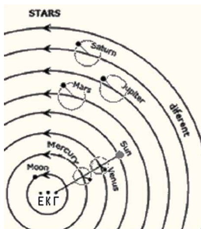
Figure 5. The cosmological model of Ptolemy. K is the centre of the deferent circles , E is the equal point and \Gamma is the centre of the Earth.
