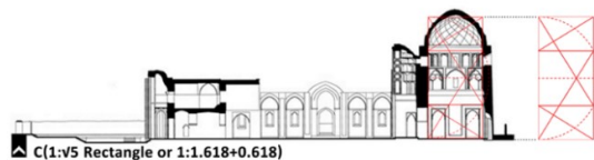
Figure 14. Golden ratio in the dome (North-south section)
