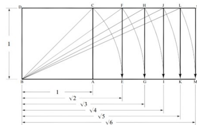
Figure 5. Dynamic rectangle
